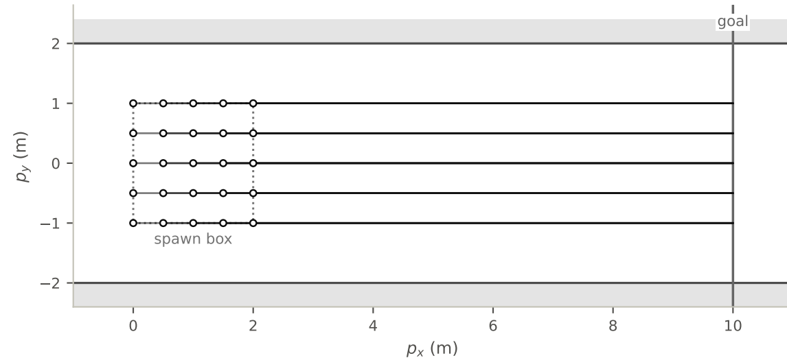
PPO, seed 19 (final.pt), same starts: 25/25 reach the goal, +0.3 steps vs the oracle on average, 0 contacts
