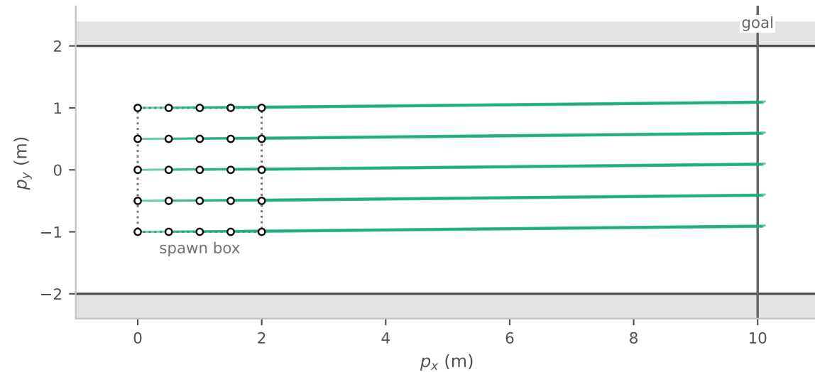
PPO+MPC, seed 2 (final.pt), same starts: 25/25 reach the goal, +0.2 steps vs the oracle on average, 0 contacts
