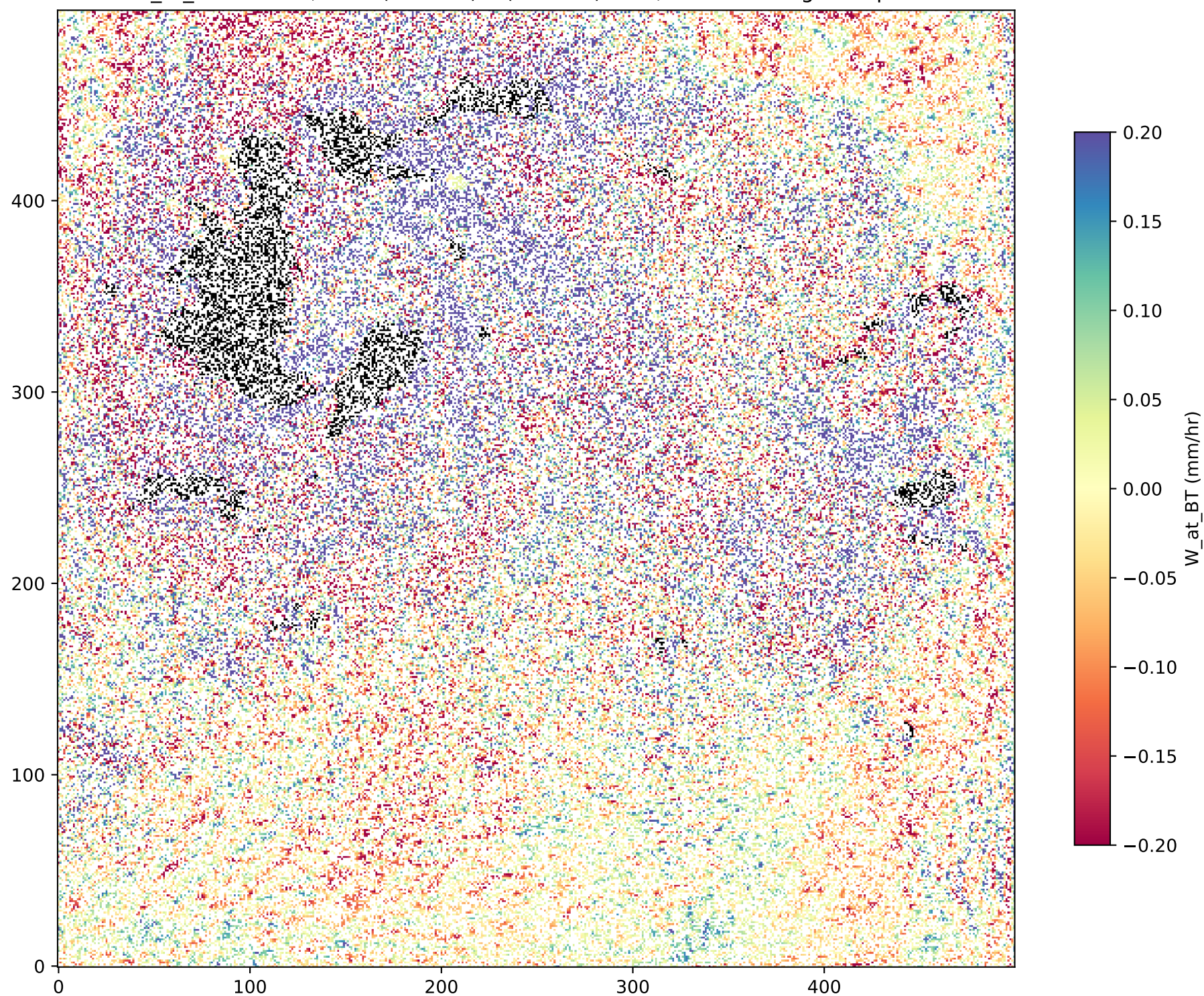
W_at_BT at t=80, filter (183 \pm 1) > (183 \pm 7) - 20 , 60\% training data points
