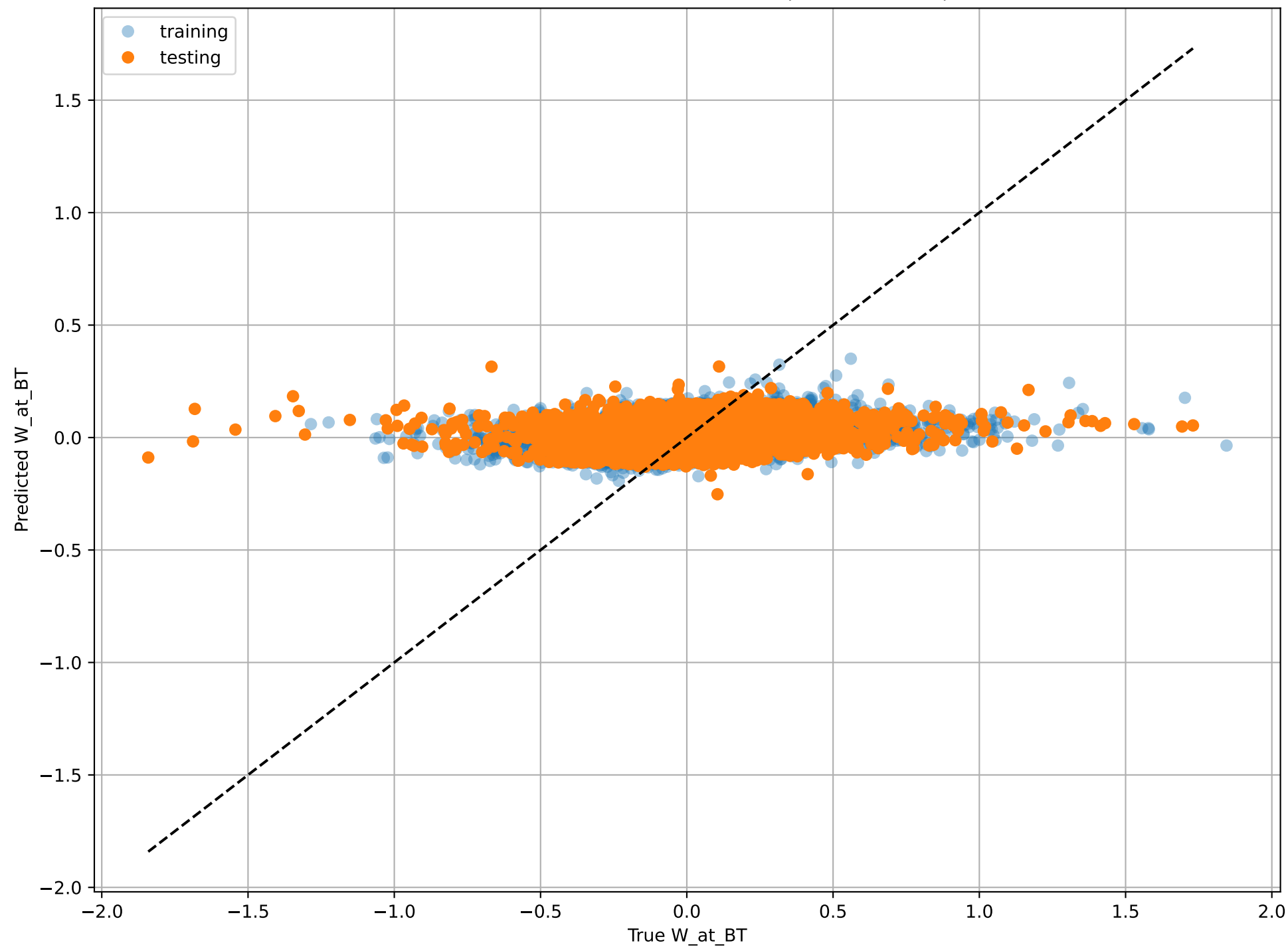
True vs Predicted with Tensorflow (score=0.1496)
