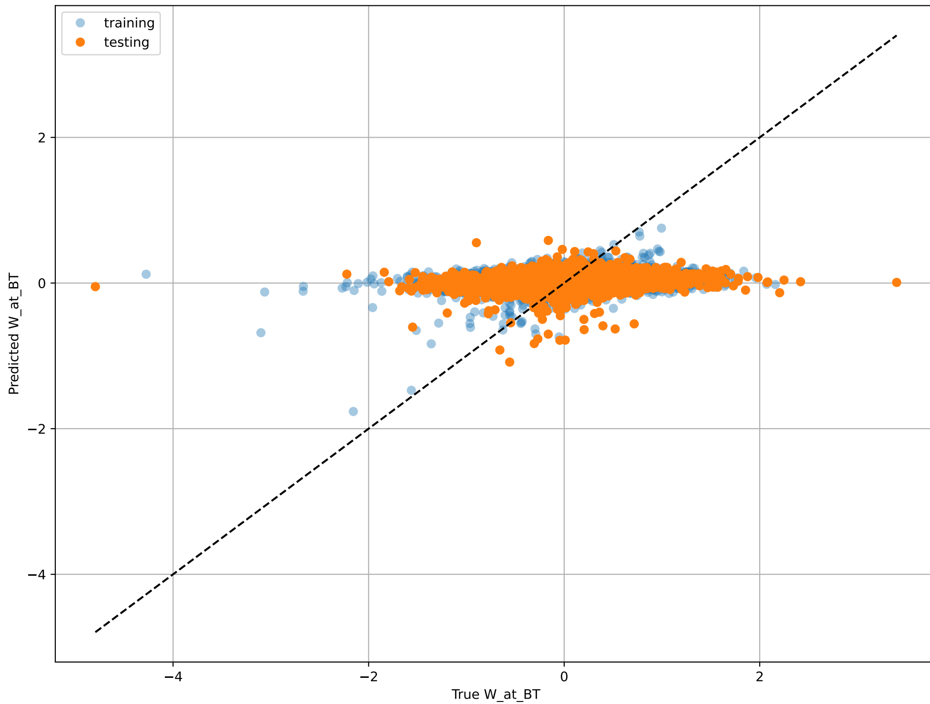
True vs Predicted with Tensorflow (score=0.0473)
