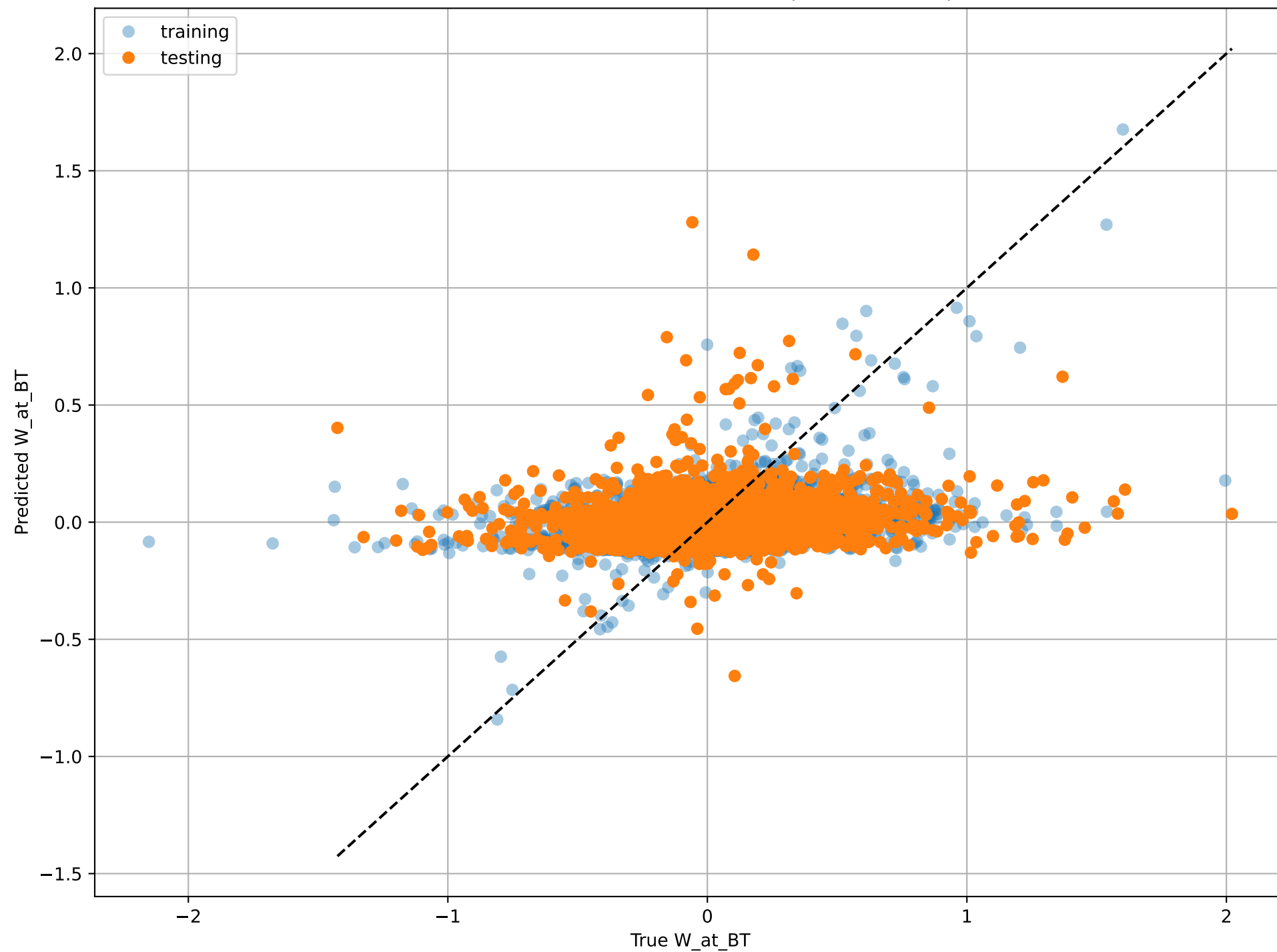
True vs Predicted with Tensorflow (score=0.0514)
