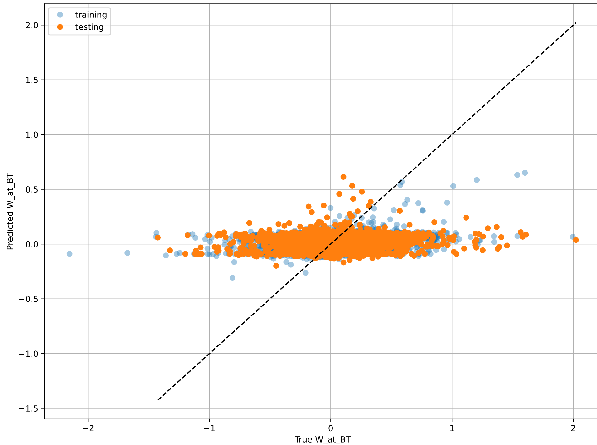
True vs Predicted with Tensorflow (score=0.0495)
