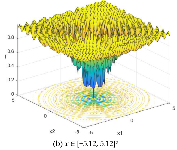
Figure 37: Drop-Wave function in two dimensions.
