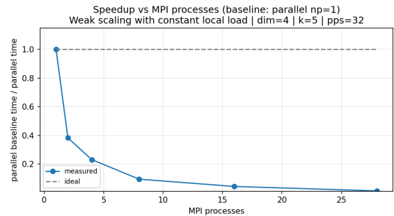
Figure 20: Hybrid Weak Scaling
