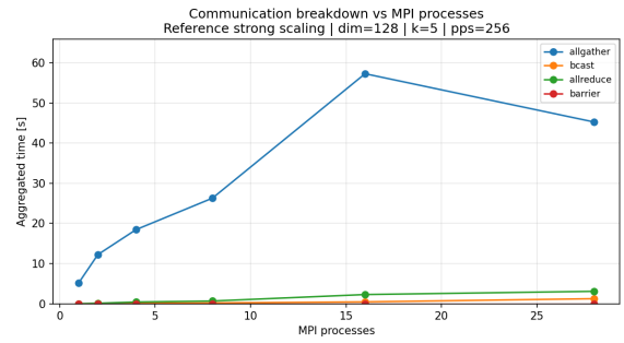
Figure 22: Communication overhead breakdown for D = 128 .
