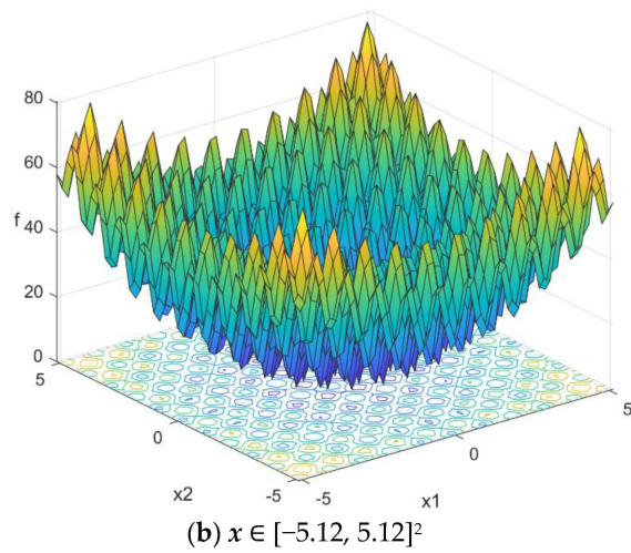
Figure 38: Rastrigin function in two dimensions.
