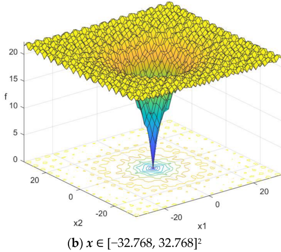
Figure 36: Ackley function in two dimensions.
