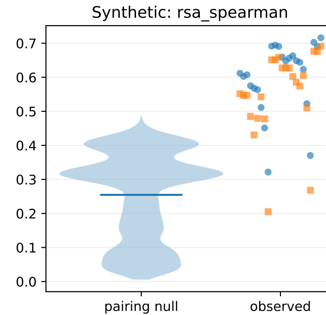
A/B correspondence vs complete-trial B-identity derangement (1000 permutations)
