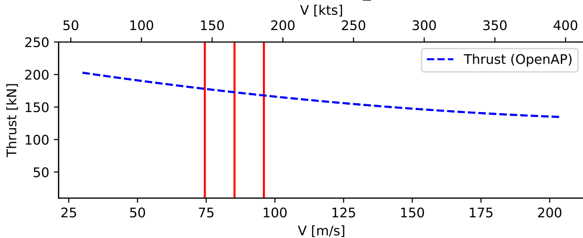
Thrust vs. speed - C_L = 1.61
