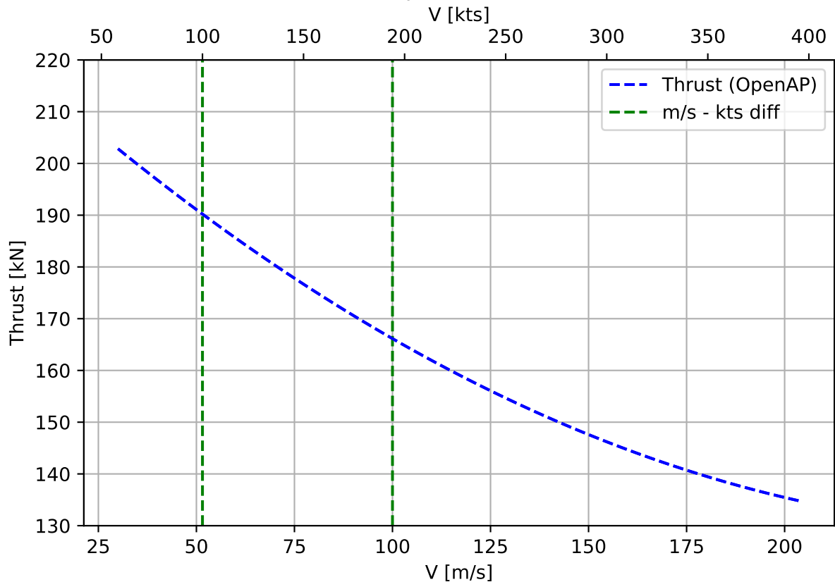
Thrust vs. speed - Altitude = 0 ft
