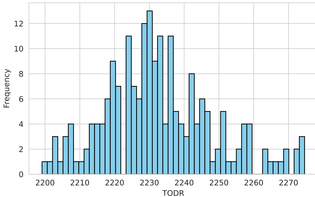
Historical Scenario
