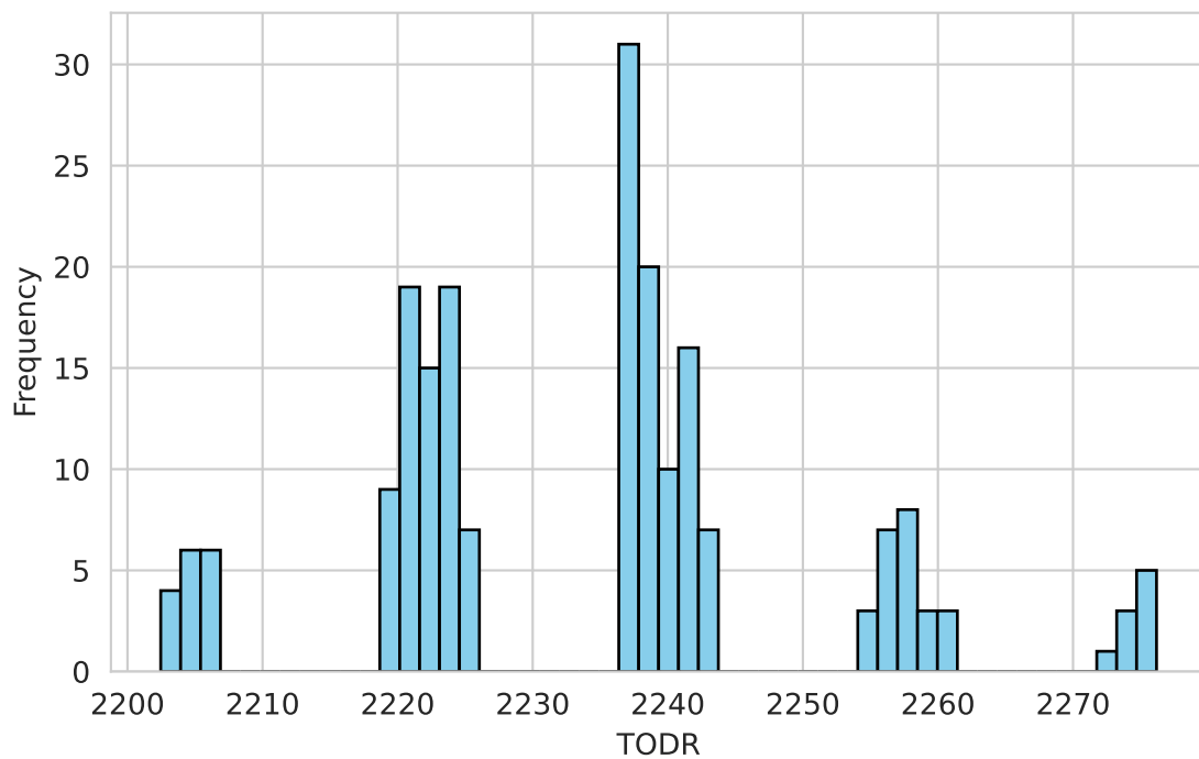
Historical Scenario
