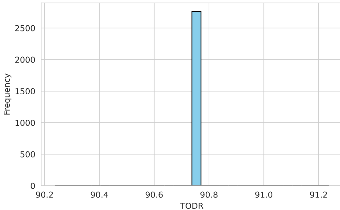
Historical Scenario
