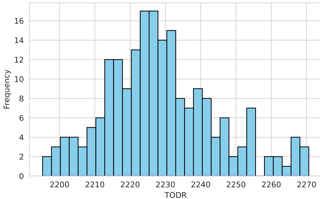
Historical Scenario
