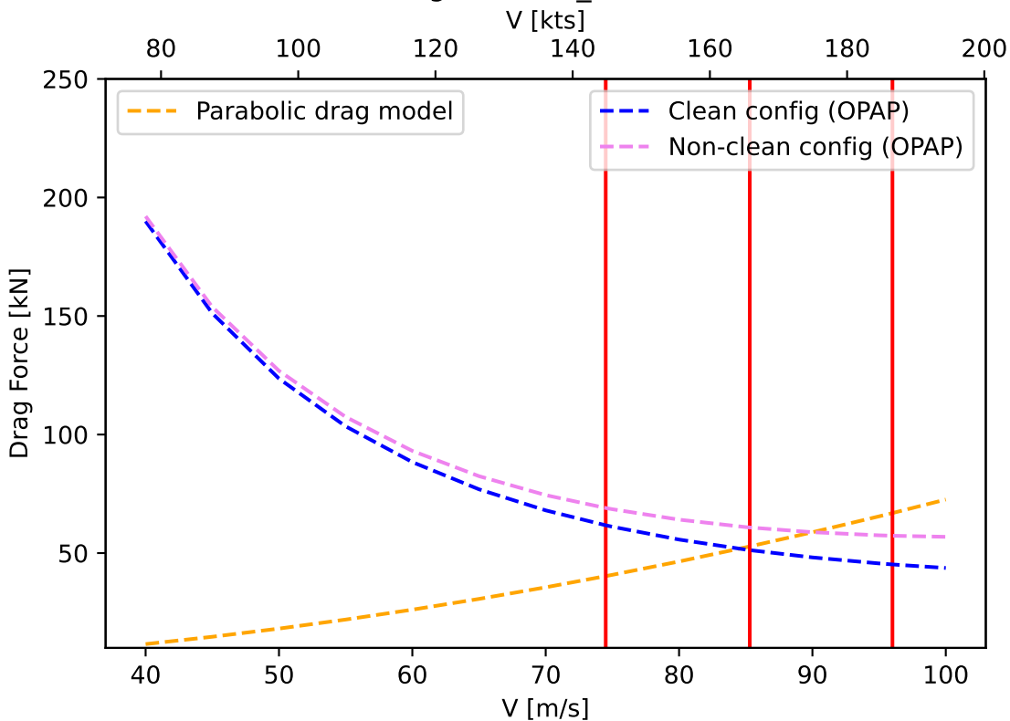
Drag vs. V - C_L = 1.41
