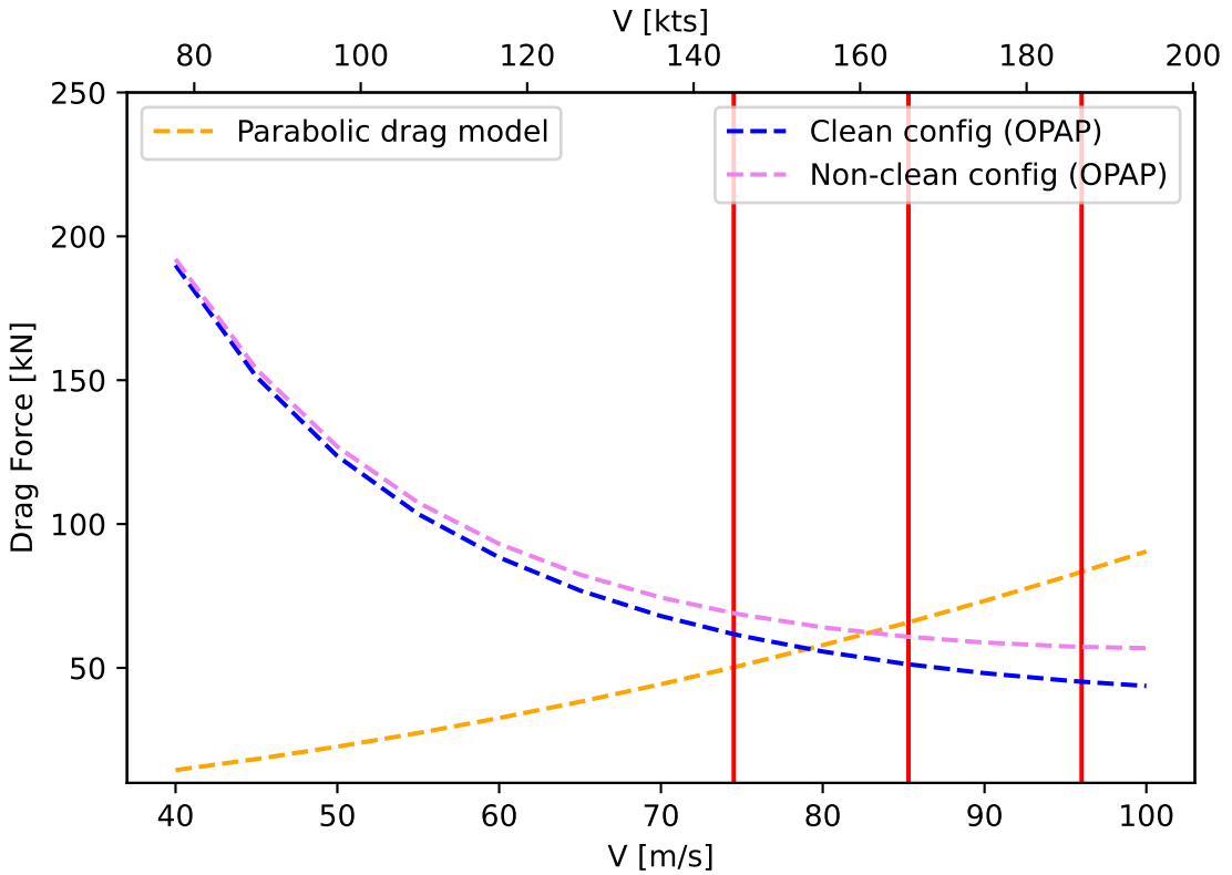
Drag vs. V - C_L = 1.61
