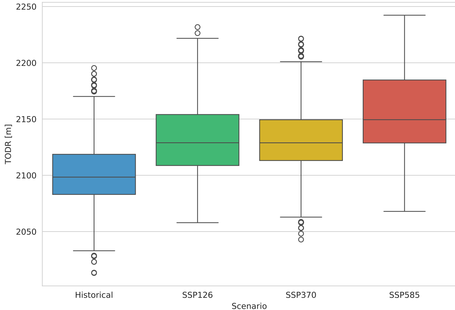
Computed Take-Off Distance Required (TODR) (JJA Data)
