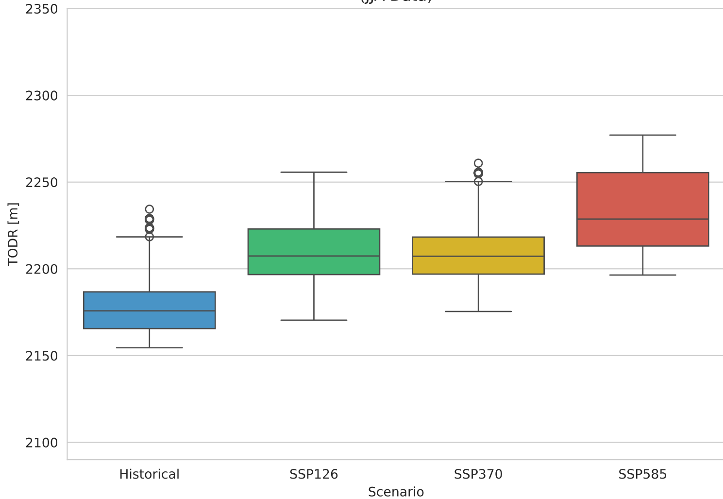
Computed Take-Off Distance Required (TODR) (JJA Data)
