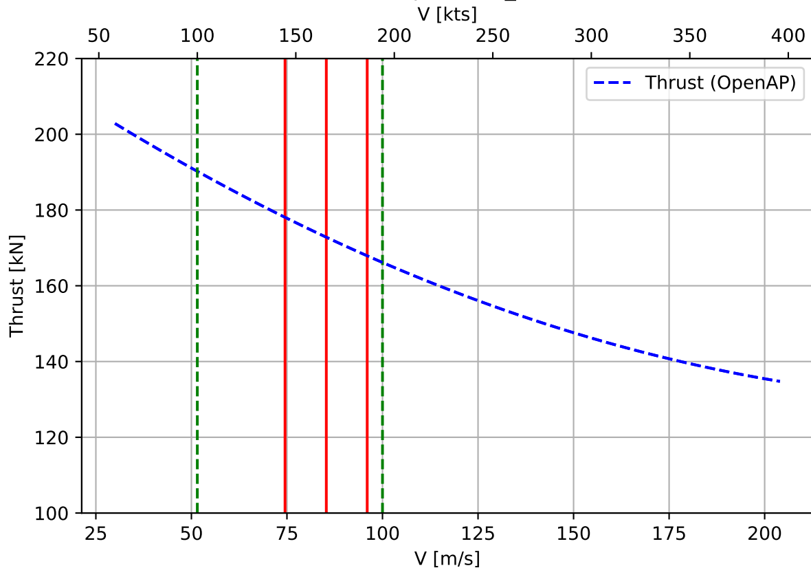
Thrust vs. speed - C_L = 1.61
