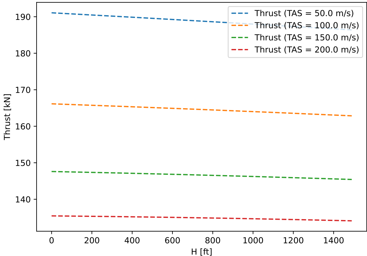
Thrust vs. elevation
