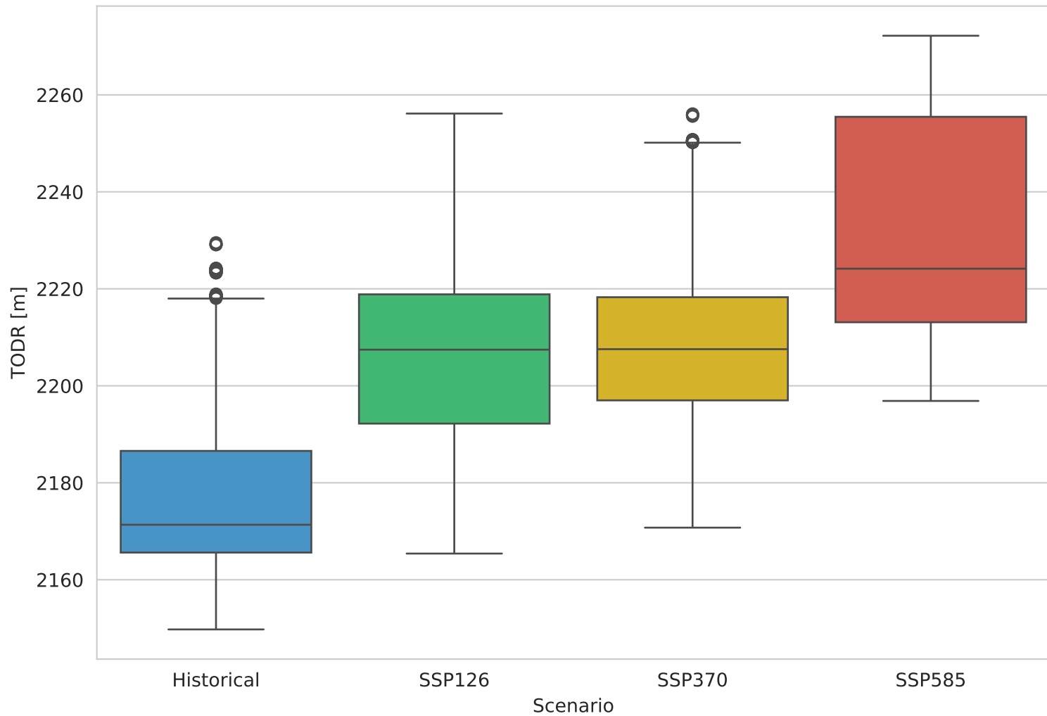
Take-Off Distance Required (TODR) (JJA Data) - EBBR - QDM
