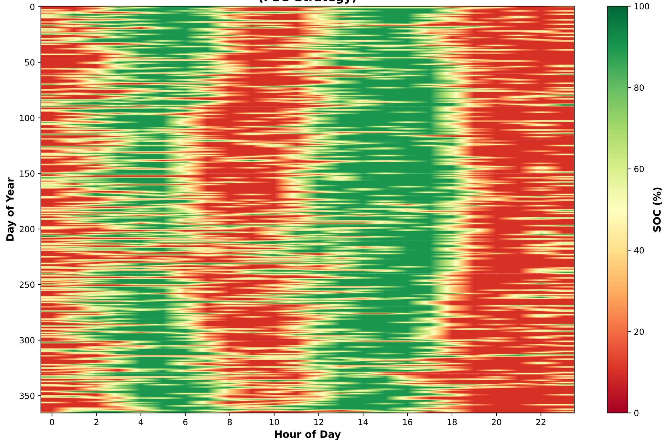
Battery State of Charge - ORNSTEIN-UHLENBECK (PSO Strategy)
