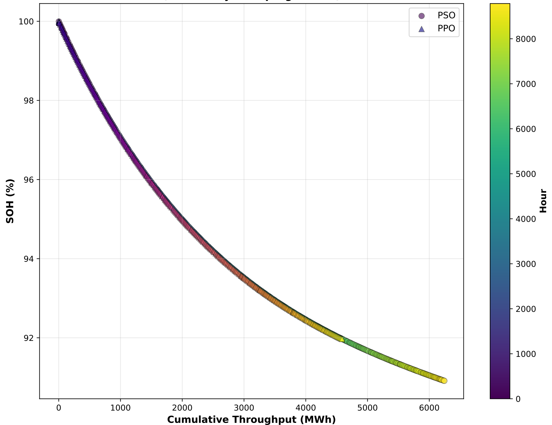
SOH vs Throughput - ORNSTEIN-UHLENBECK (Colored by time progression)
