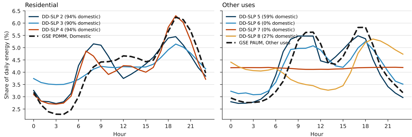
Daily shapes, winter weekday, each family against its own national profile
