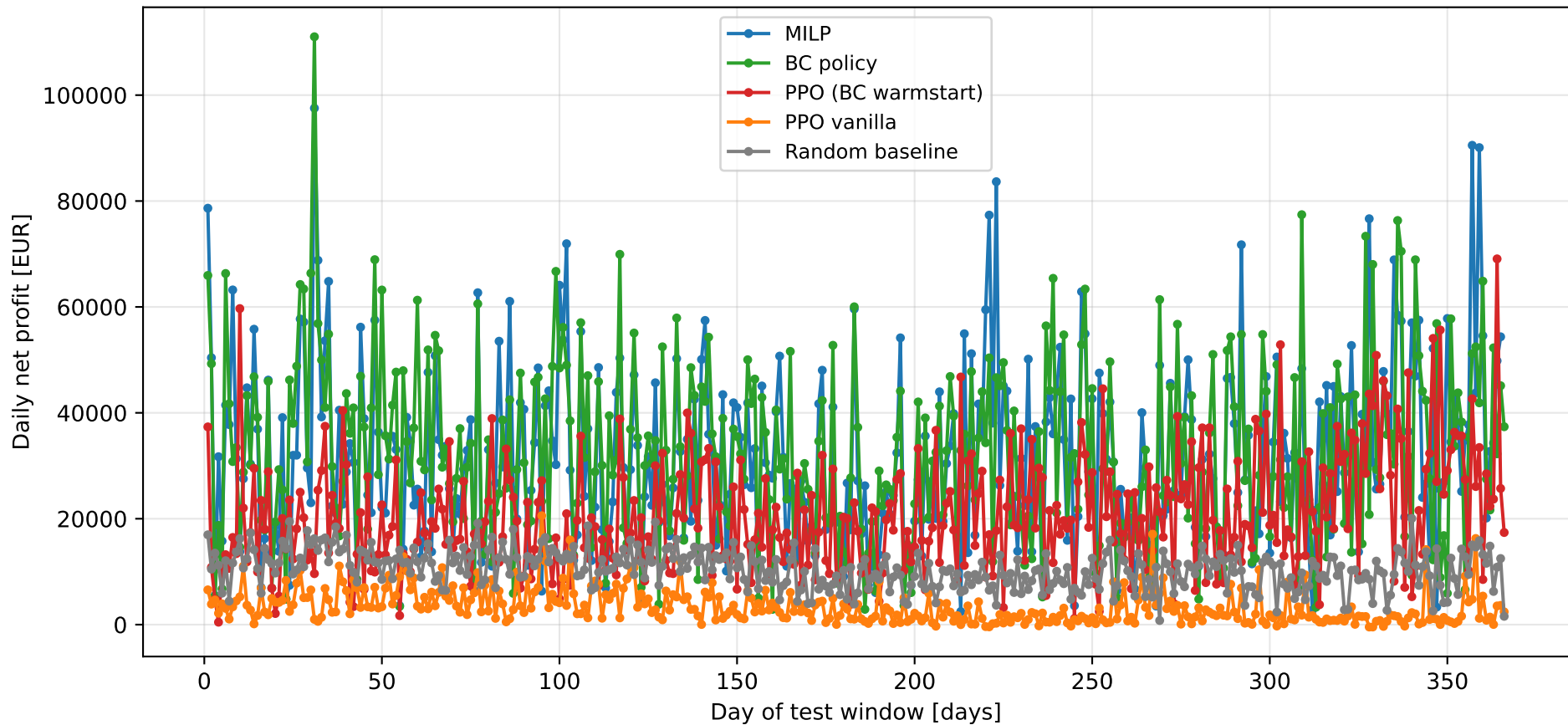
Daily net profit by policy on test window
