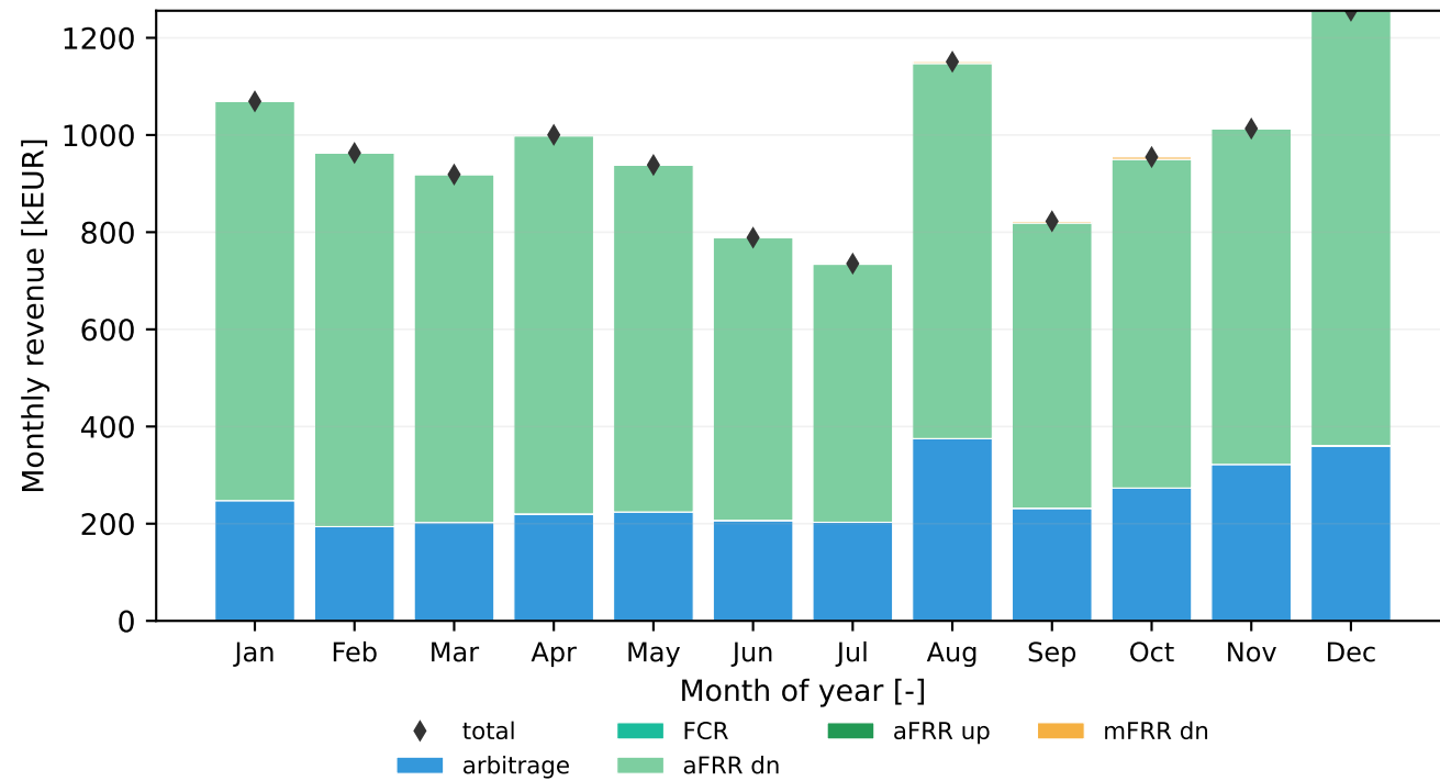
MILP
