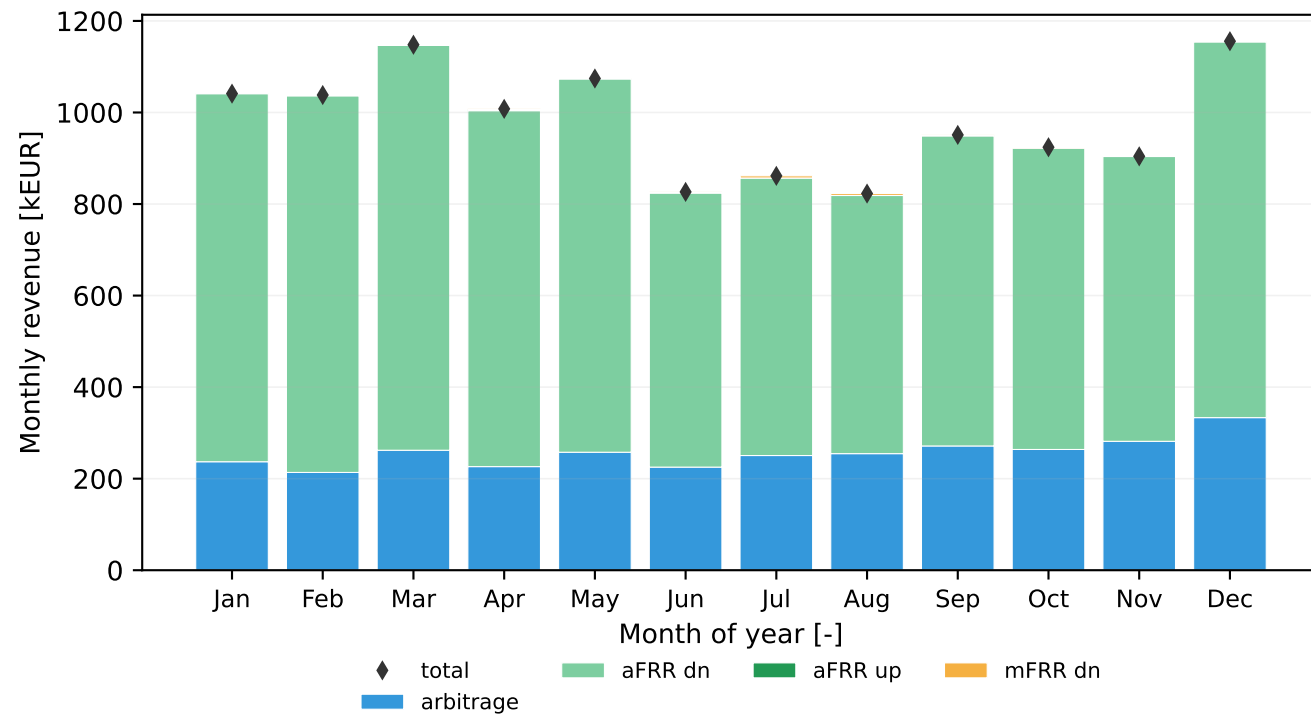
MILP
