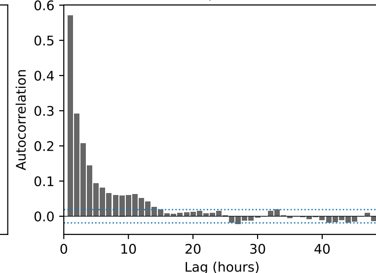
ACF — \rho_1 = 0.571
