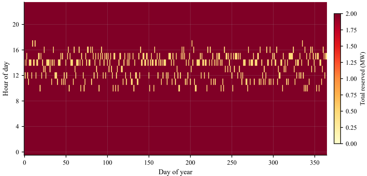
MILP: total flexibility reservation (MW) (normal)
