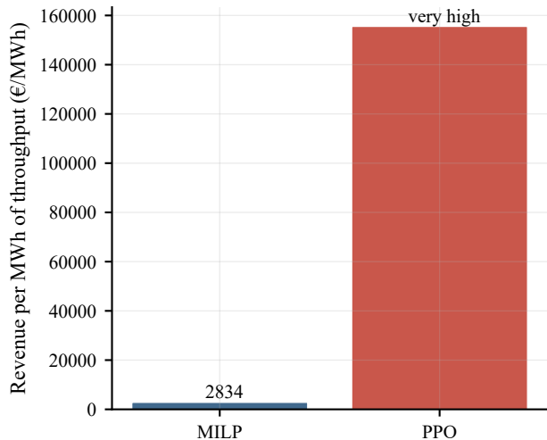
Economic efficiency
