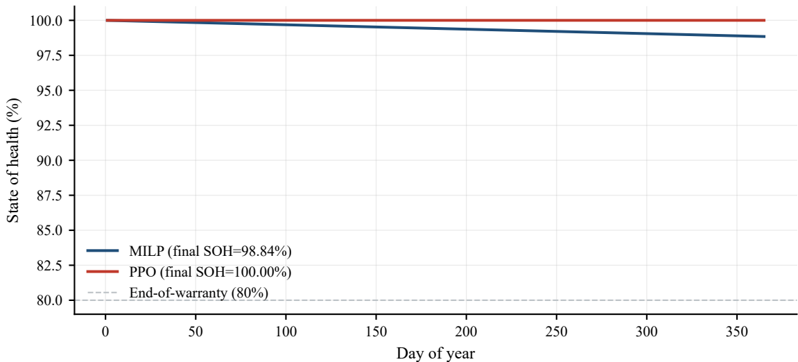
Cumulative cycle aging (linear LCOS model) (fixed-bias)
