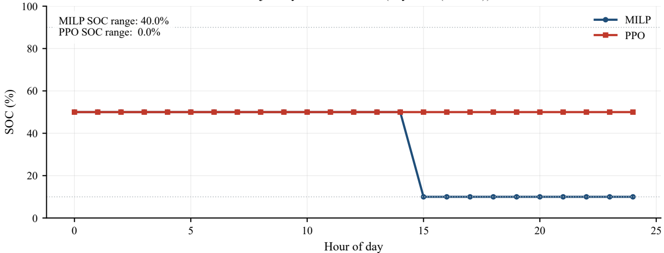
SOC trajectory: MILP vs PPO (day 267 (normal))
