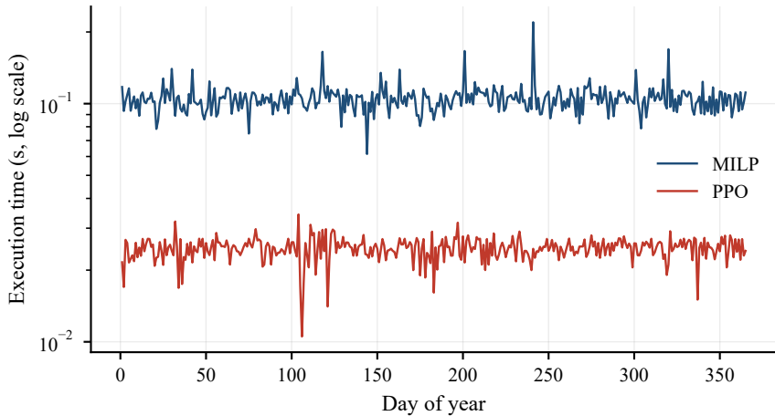
Daily execution time per 24-hour horizon (fixed-bias)
