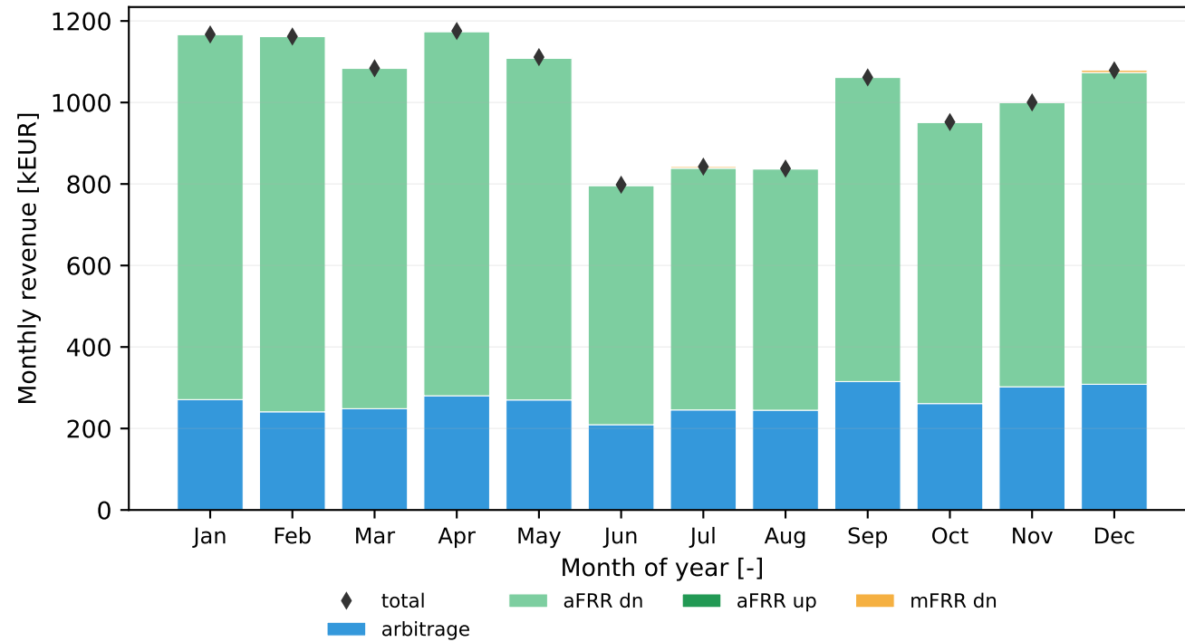
MILP
