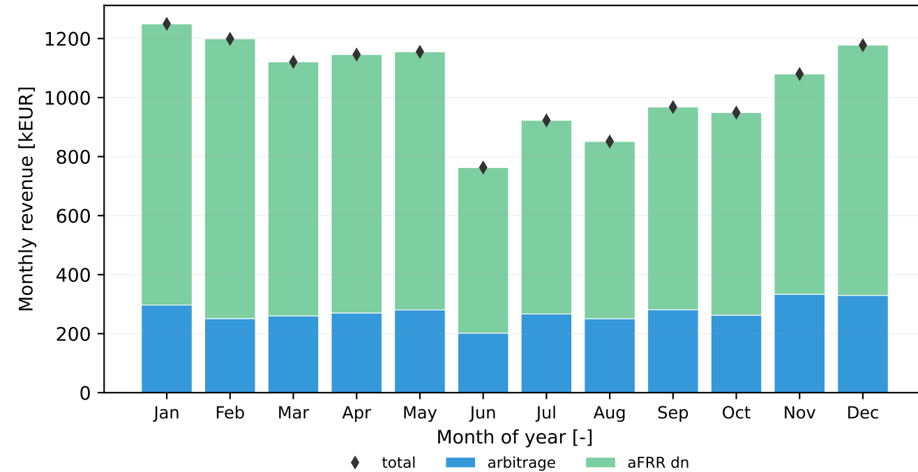
BC policy
