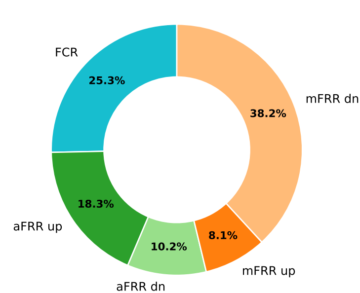
PPO vanilla Total flex: 1,960,270 EUR
