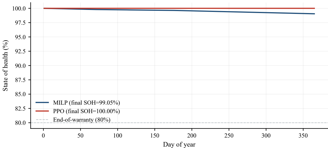
Cumulative cycle aging (linear LCOS model)
