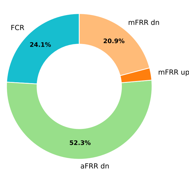
PPO vanilla Total flex: 5,829,765 EUR
