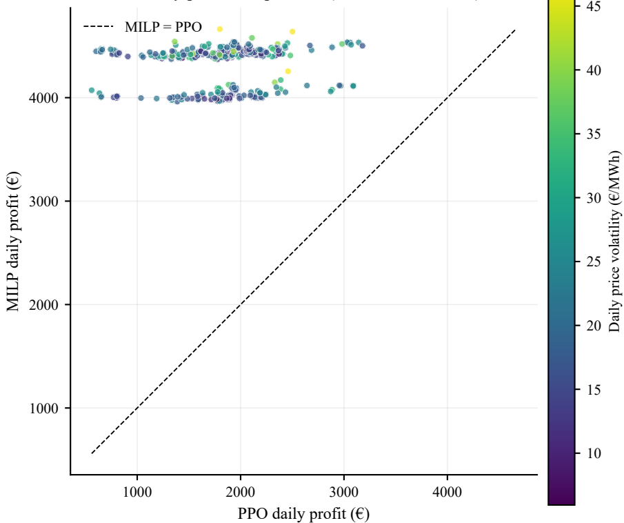
Per-day profit comparison (ornstein-uhlenbeck)
