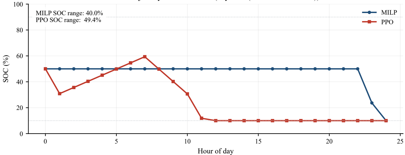
SOC trajectory: MILP vs PPO (day 163 (ornstein-uhlenbeck))
