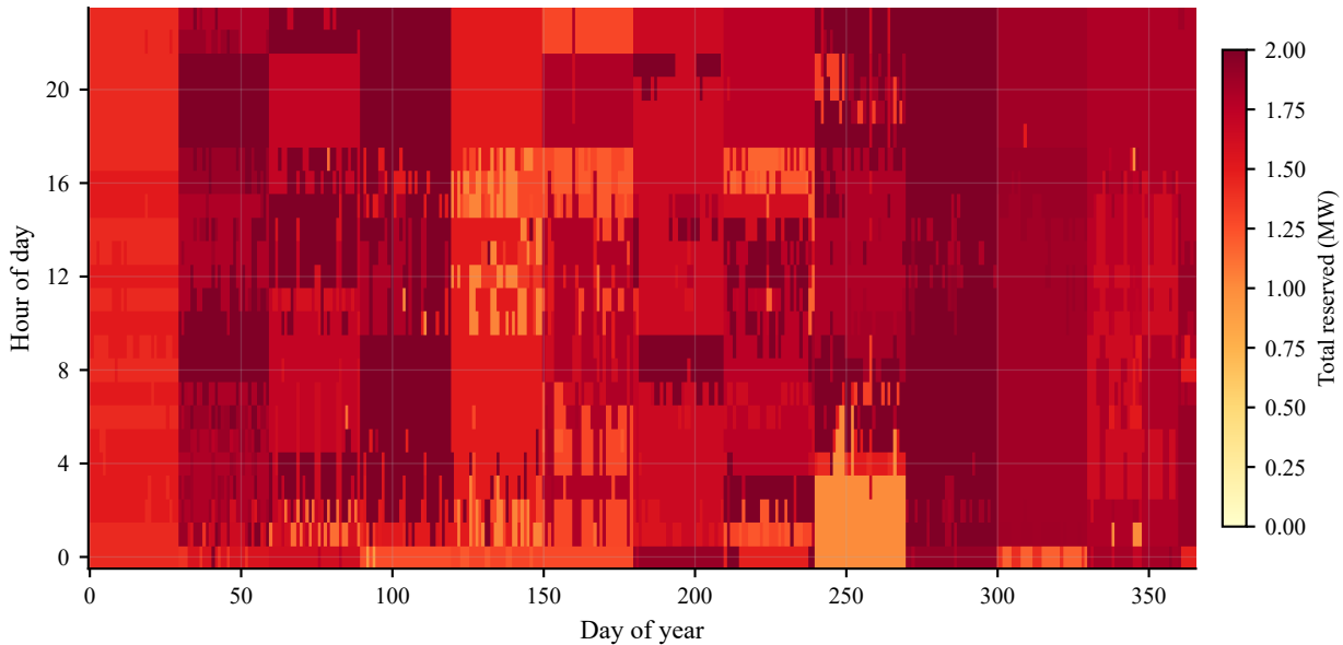
PPO: total flexibility reservation (MW) (ornstein-uhlenbeck)
