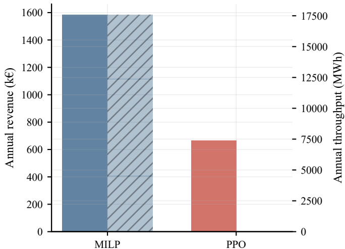
Annual revenue and throughput (ornstein-uhlenbeck)
