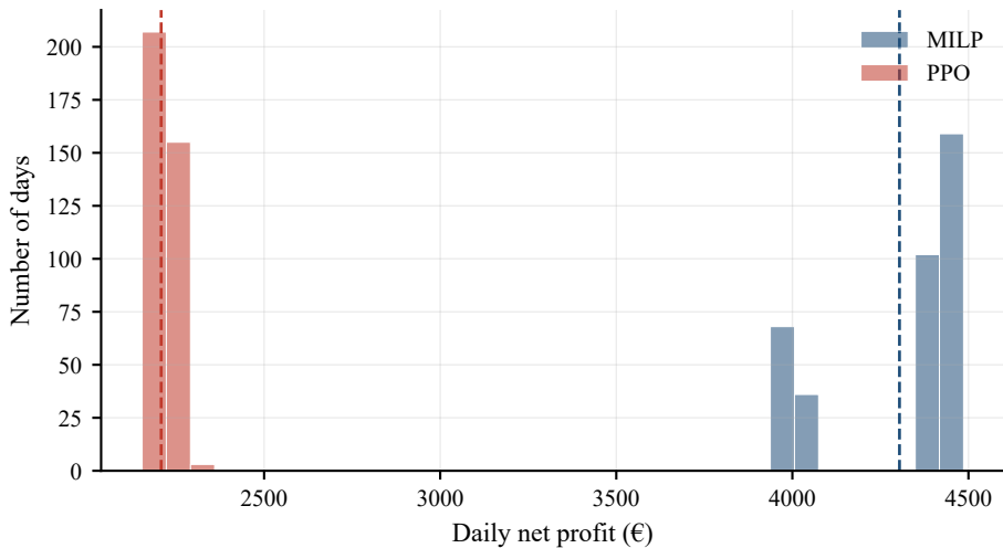
Daily profit distribution (ornstein-uhlenbeck)
