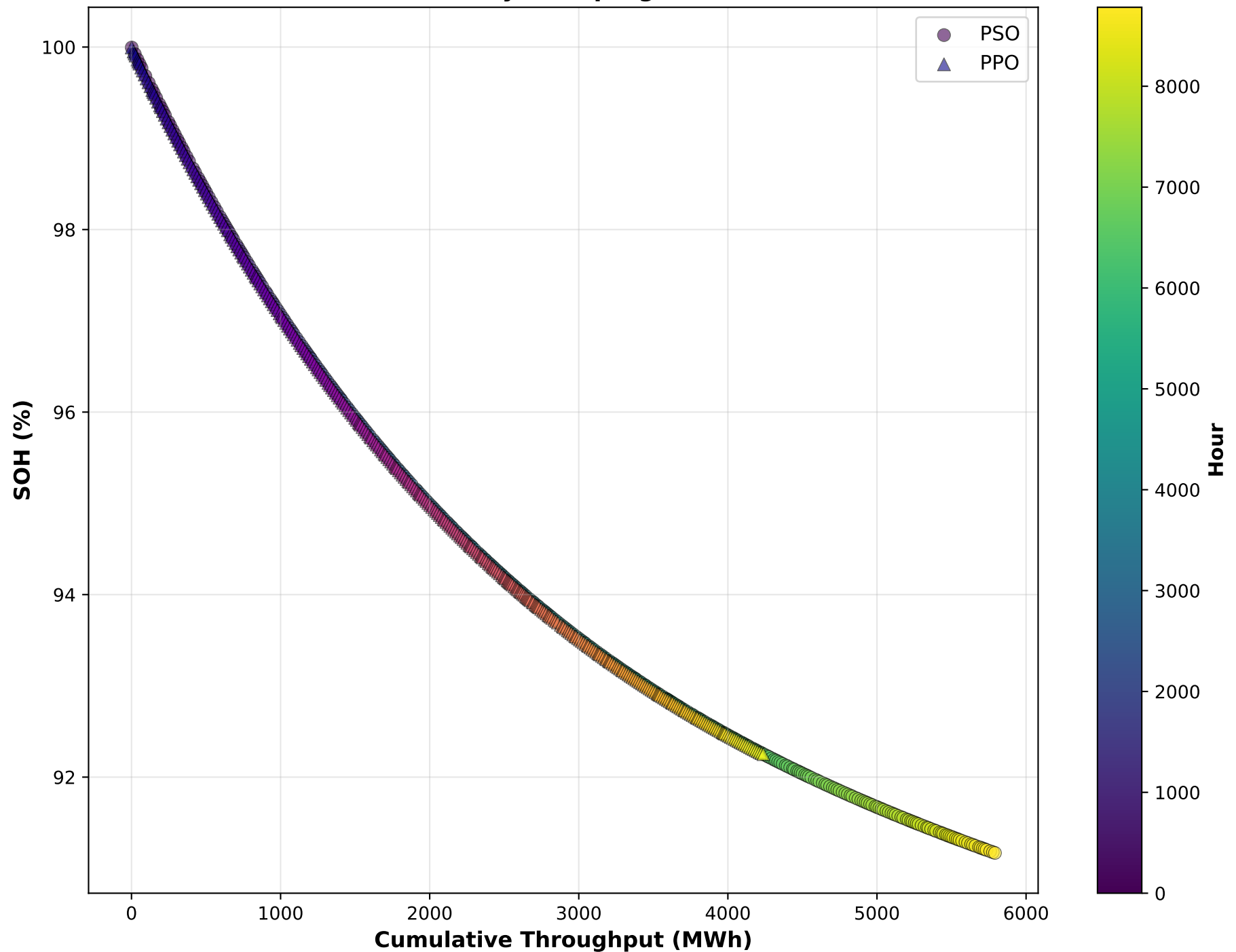
SOH vs Throughput - NORMAL (Colored by time progression)
