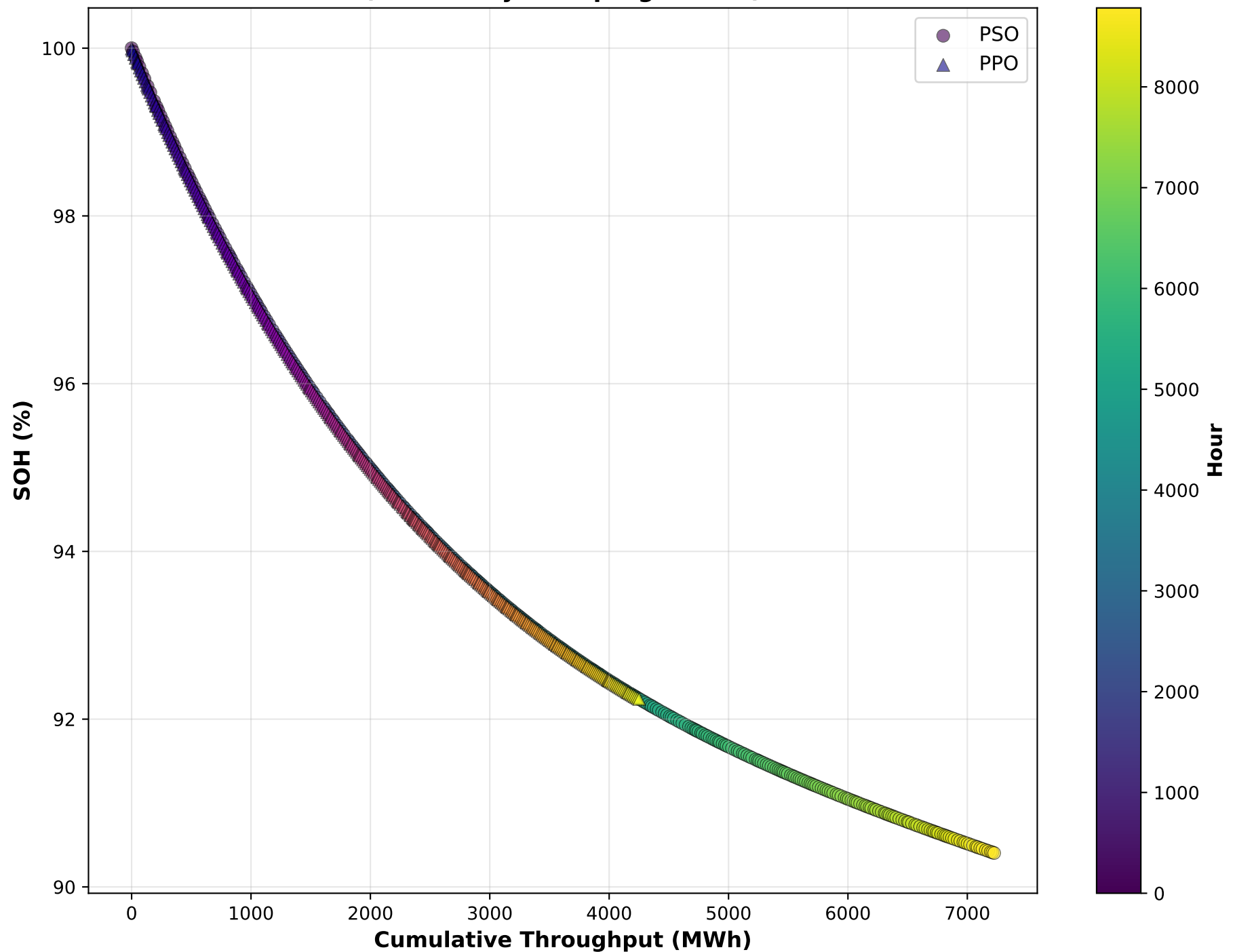
SOH vs Throughput - UNIFORM (Colored by time progression)
