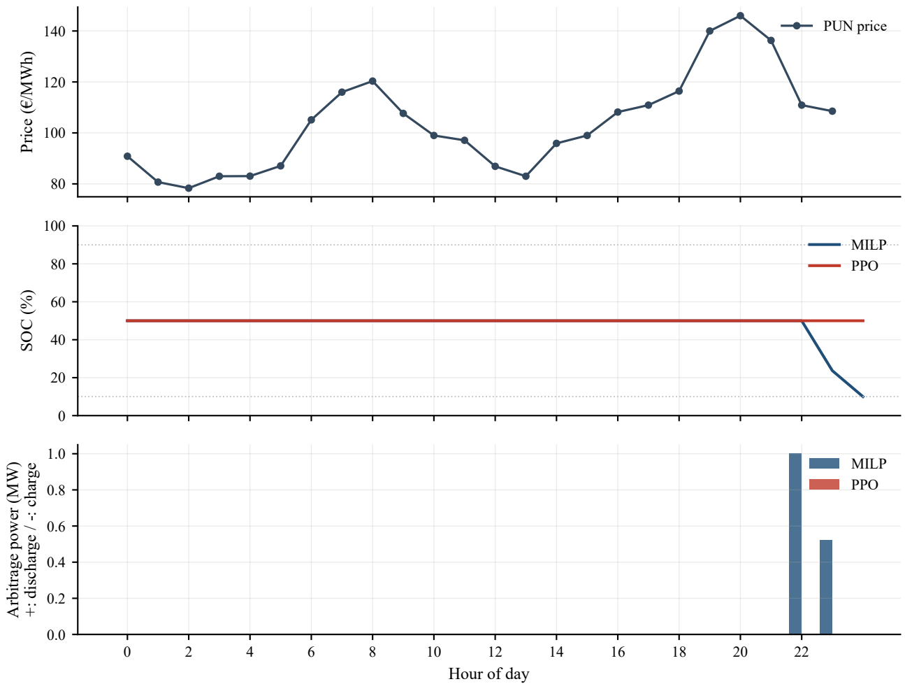
Representative day 163: price, SOC and power
