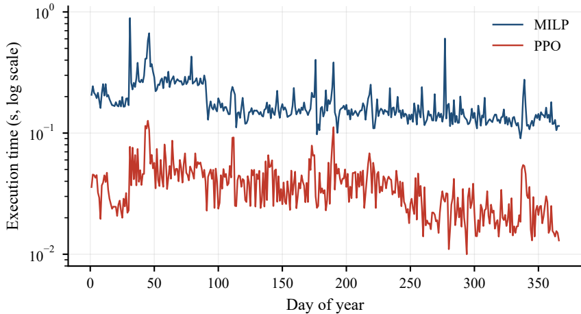
Daily execution time per 24-hour horizon (ornstein-uhlenbeck)
