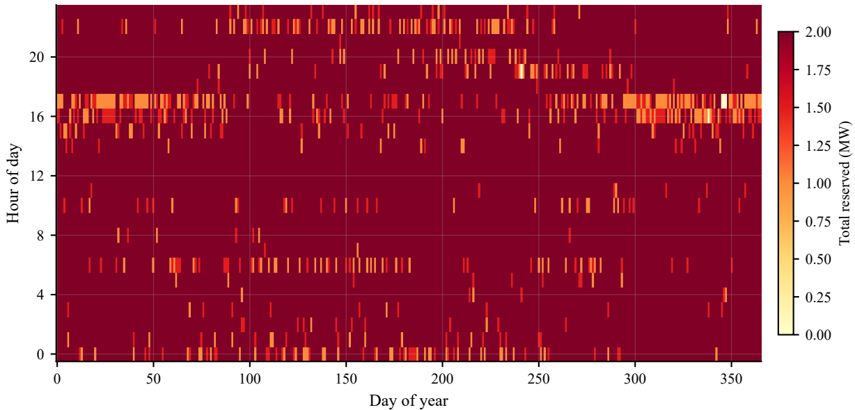
MILP: total flexibility reservation (MW) (ornstein-uhlenbeck)
