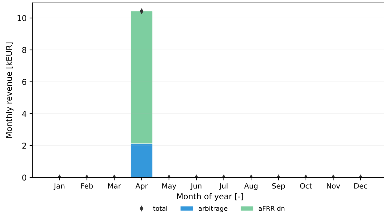
MILP
