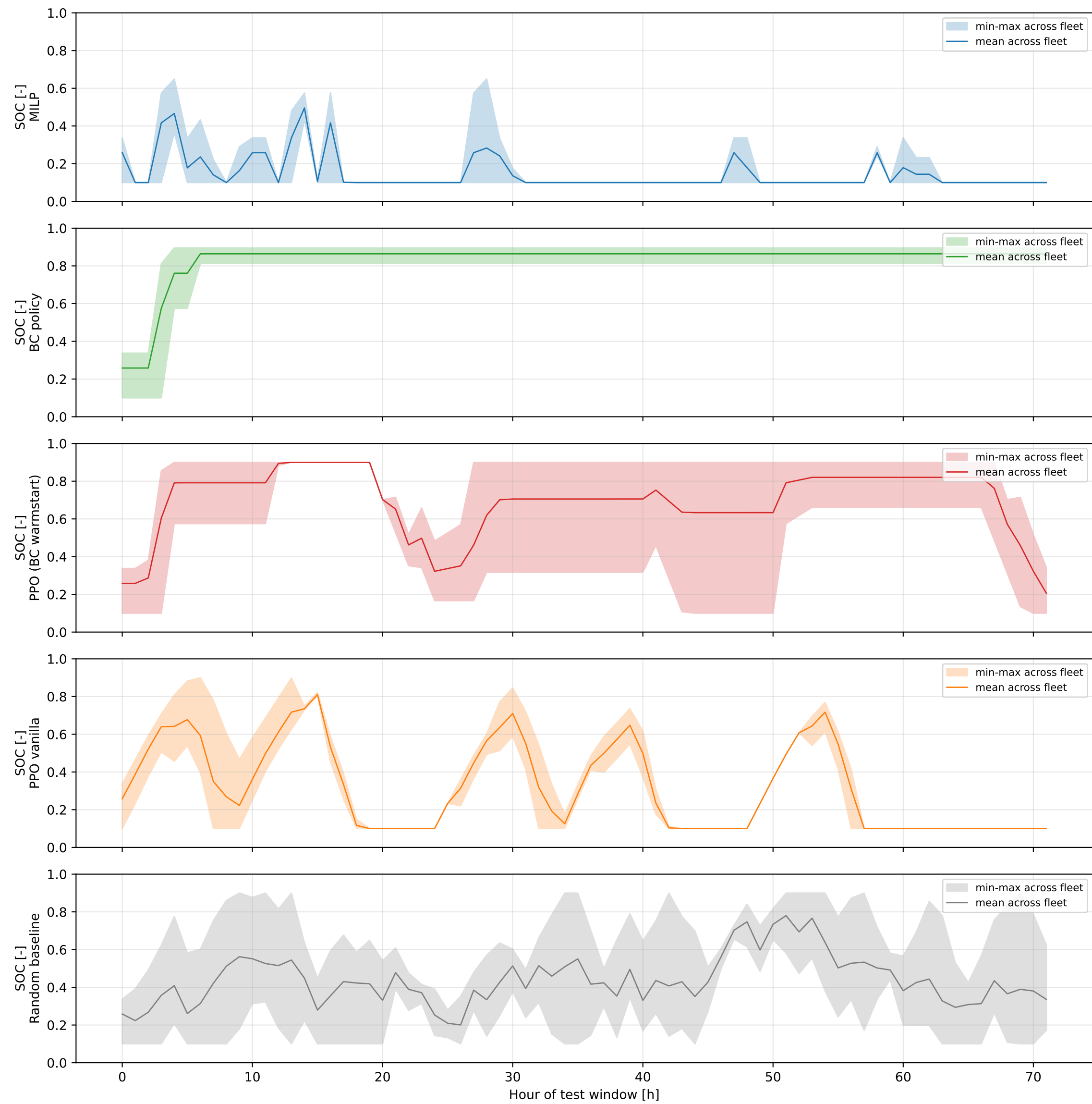
Fleet-wide SOC trajectory by policy
