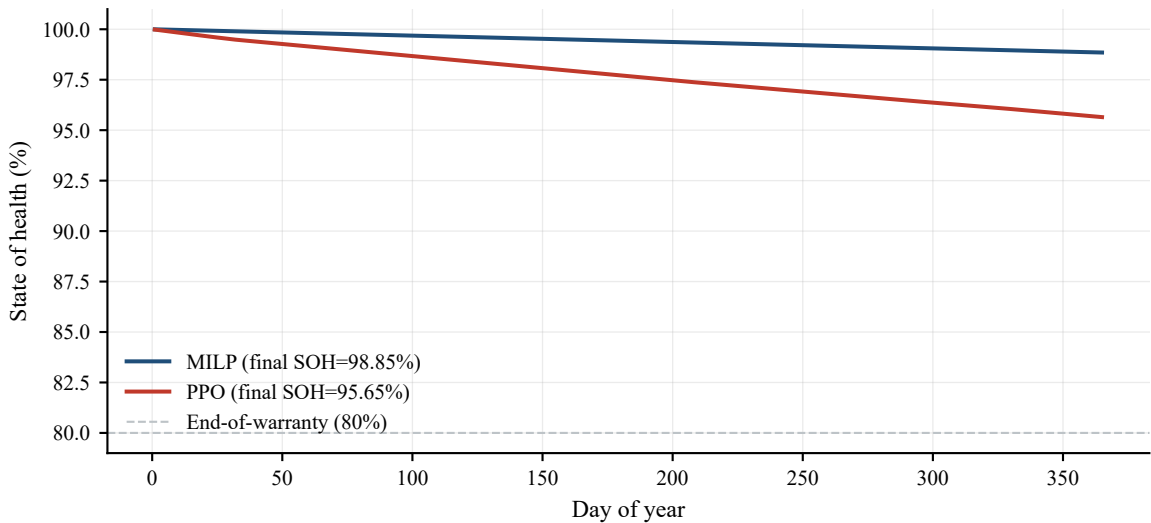
Cumulative cycle aging (linear LCOS model) (normal)
