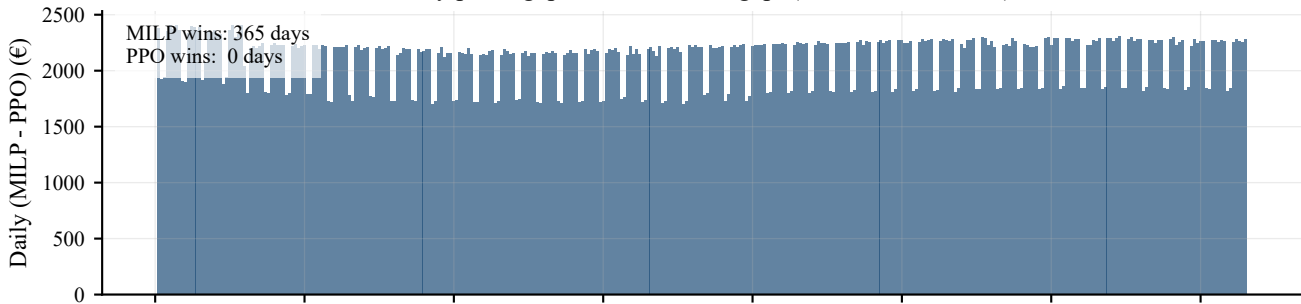
Daily profit gap and cumulative gap (ornstein-uhlenbeck)
