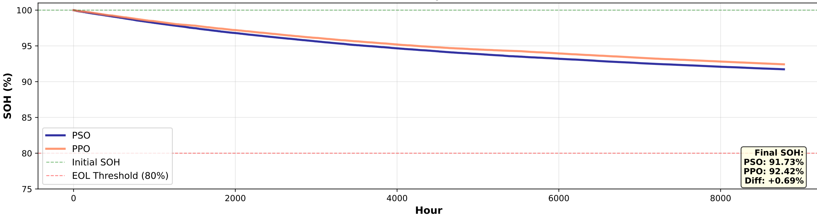
State of Health Comparison - NORMAL
