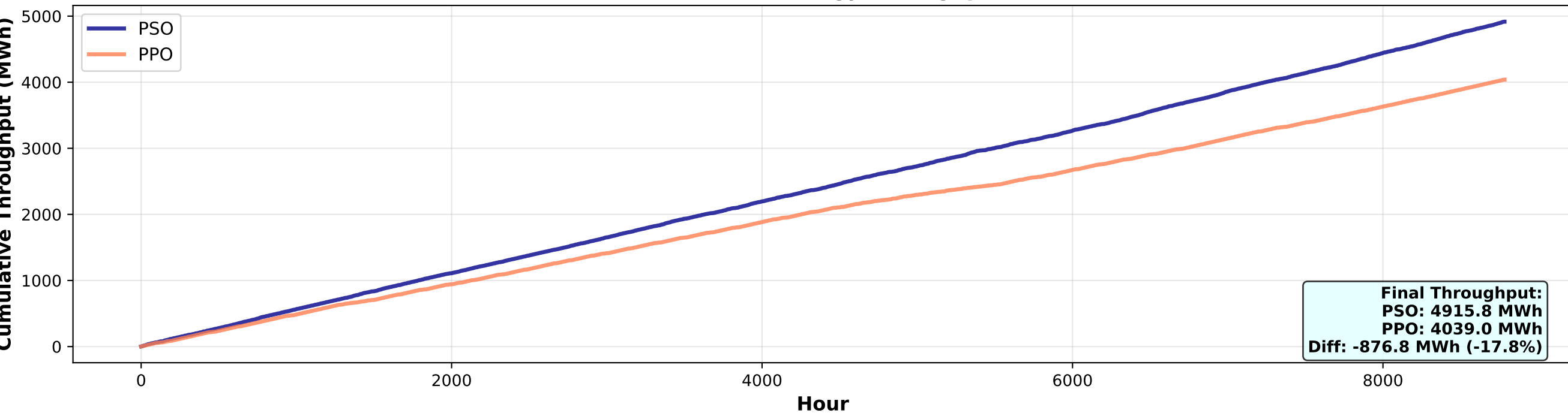
Cumulative Energy Throughput
