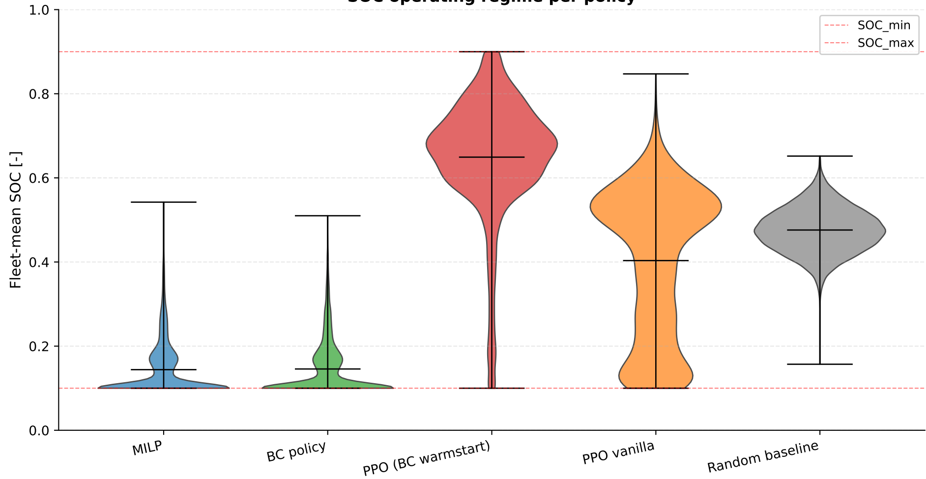
SOC operating regime per policy
